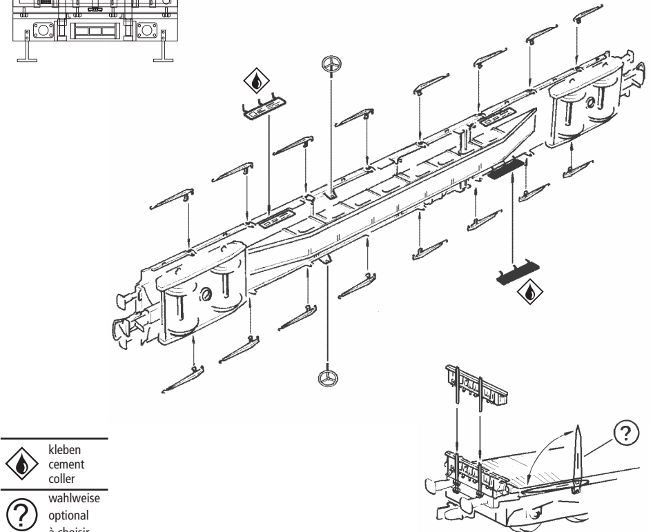
ROCO Oiler 10906
